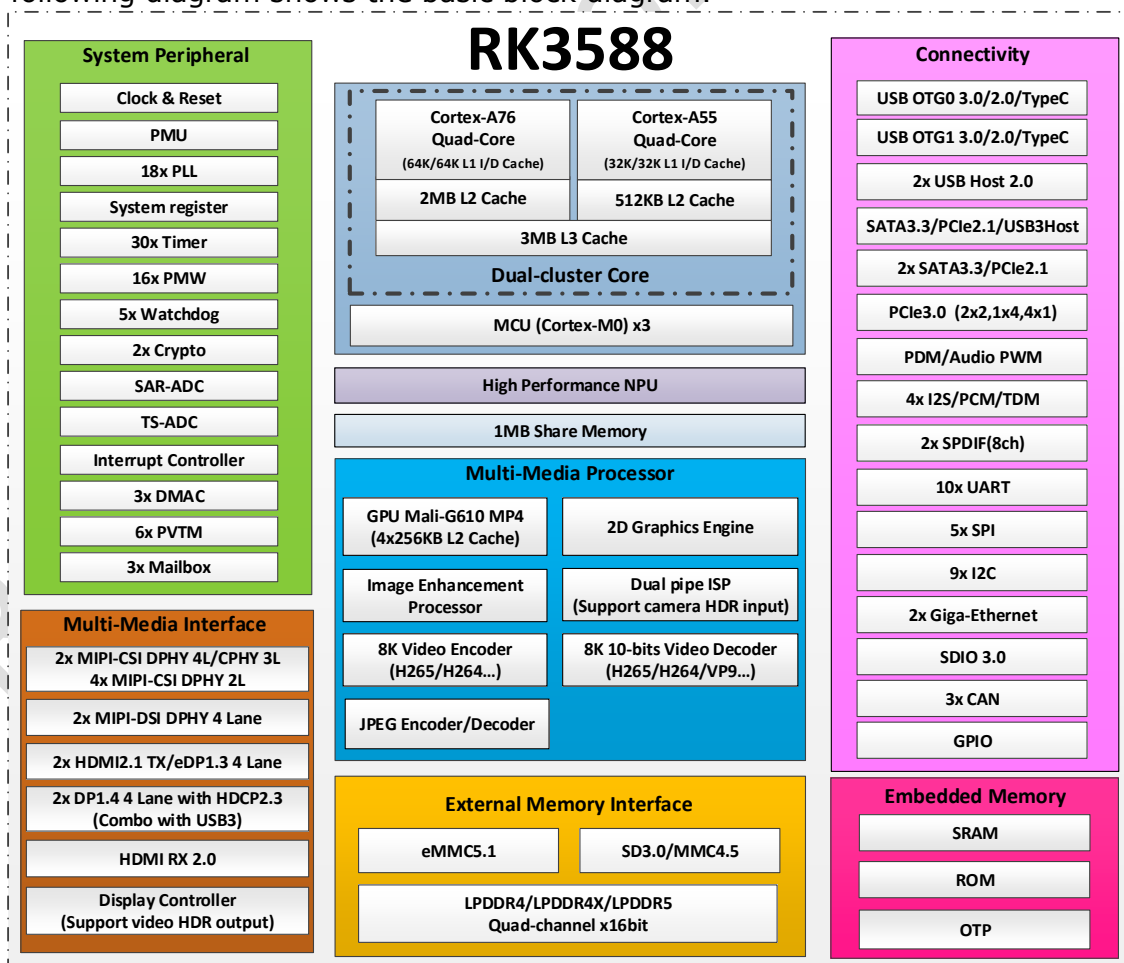
Fig.1-1 Block Diagram
