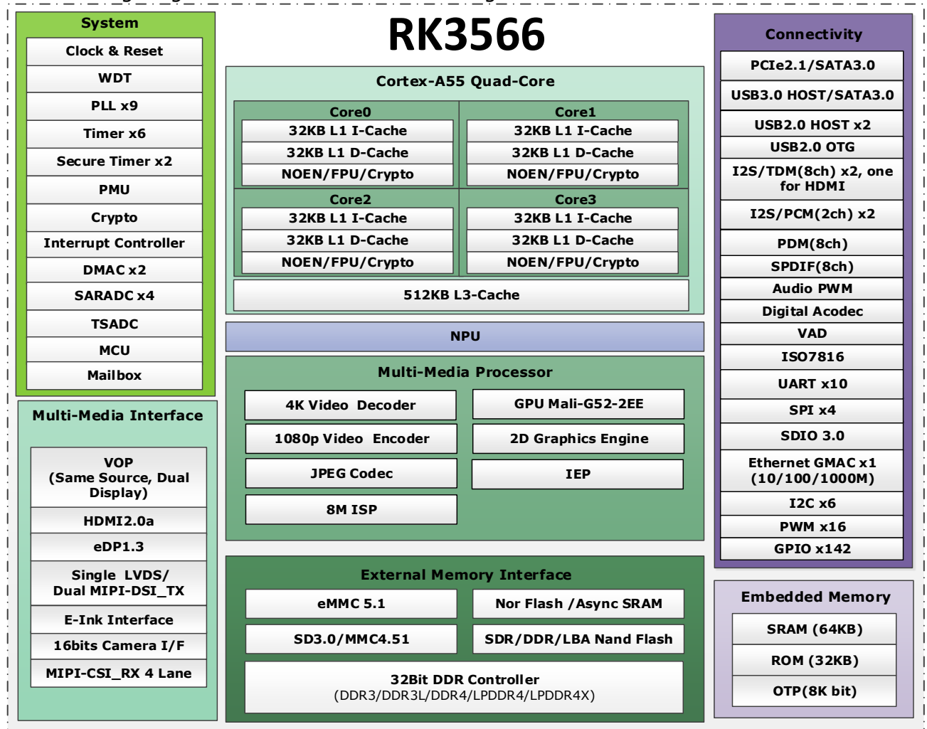
Fig.1-1 Block Diagram
