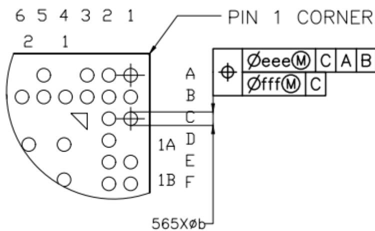
DETAIL B(2:1)
