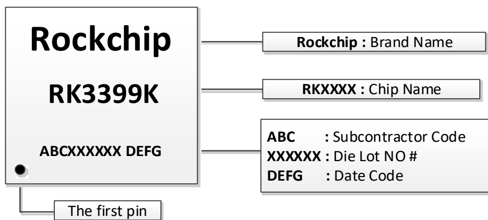
Fig. 2-2RK3399K Top Marking
